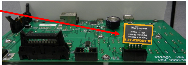
BL-1000MEXP-1011 Installed Back of BaseStation 1000 Display
