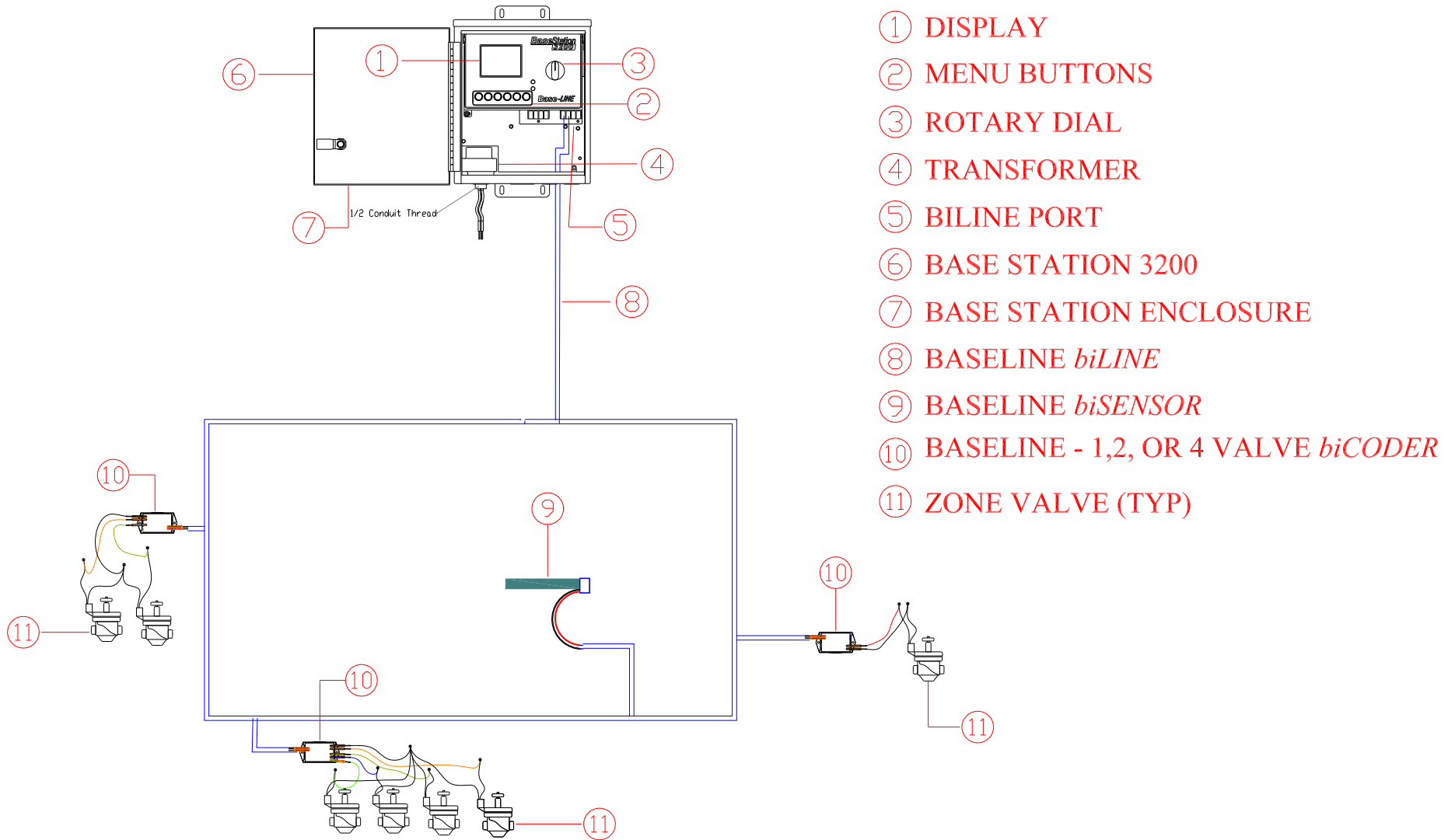
BASESTATION 3200 SITE CONTROLLER WITH ENCLOSURE LAYOUT NTS
